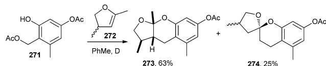
Scheme 57 Synthesis of benzopyran 273 and mono-benzannulated spiroketal 274.
