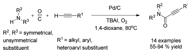
Scheme 42 Reagents and conditions: alk-1-yne (1 mmol), secondary amine (1.5 mmol), 10% Pd/C (8 mol%), CO/ \text{O}_2 pressure (5/1 atm), TBAI (0.90 mmol), 1,4-dioxane (10 mL), temperature 80 °C, time 14 h.
