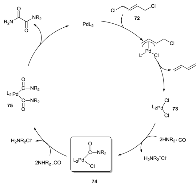
Scheme 84 Proposed mechanism for the catalytic carbonylation of a secondary amine to form an oxamide with DCB as a Pd oxidant.
