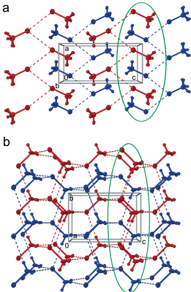
Fig. 5 Two layers of \text{Br}\cdots\text{Br} bonded \text{CH}_3\text{Br} molecules in phase \alpha (a) and two interweaved diamondoid \text{C}\text{--}\text{H}\cdots\text{Br} bonded networks of phase \beta (b), shown in autostereographic projections. 49 Dashed lines indicate the shortest intermolecular contacts (cf. Table 2). The layers in \alpha\text{-CH}_3\text{Br} (a) are coloured red ( y = 0.75 ) and blue ( y = 0.25 ); the interpenetrating 3-dimensional networks in \beta\text{-CH}_3\text{Br} (b) are discriminated by colours, too. The encircled groups of molecules correspond to the same part of the prototypic \text{Br}_2 structure, as explained in the text. The displacement ellipsoids are drawn at the 40% probability level.
