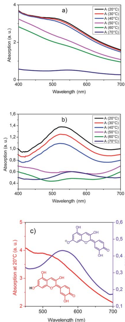
Fig. 6 Temperature dependency of the visible absorption of PLA composite I: (a) original curves on heating, (b) slope corrected curves on heating and (c) thermochromic switching effect, red curve: cold state, violet curve: hot state.
