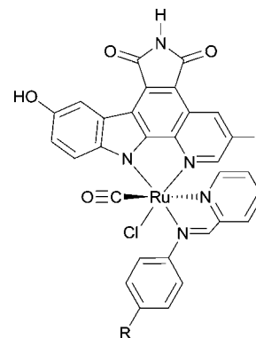
16a \text{R} = \text{H} ( \Delta -FL172) \text{IC}_{50} = 130 \text{ nM} 16b \text{R} = \text{CH}_3 ( rac -FL224) 4% inhibition at 100 nM 16c \text{R} = \text{F} ( rac -FL252) no inhibition at 100 nM
