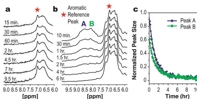
Fig. 3 Selective substitution of \beta -homo-pentafluorophenylalanine improves \beta -peptide bundle stability as judged by NMR. (a) The amide NH regions of the Acid-1Y FF and (b) Acid-1Y FF * \beta -peptide bundles after dissolution in D 2 O. In the case of Acid-1Y FF , no amide NH resonances are visible within 15 min after addition of D 2 O. In the case of Acid-1Y FF *, the amide signals persist for more than 1 h. (c) Integration of the resonances indicated in (B) normalized to the aromatic reference peak and fit to exponential decays to determine average exchange rate constants.
