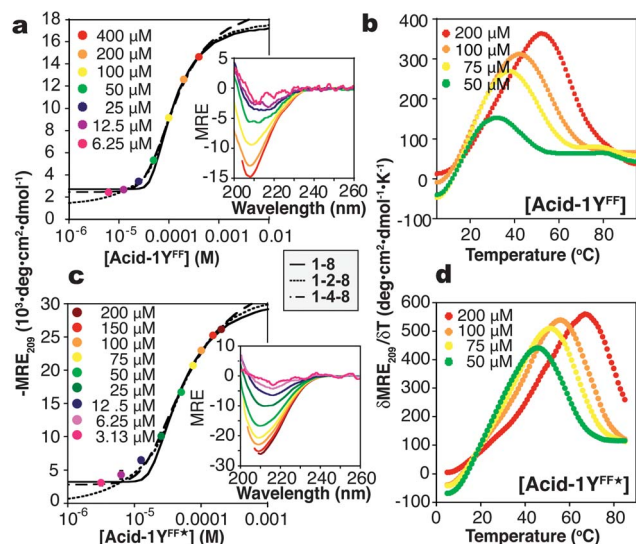
Fig. 2 Self-association of designed \beta -peptide bundles. Circular dichroism spectra of Acid-1Y FF (a and b) and Acid-1Y FF * (c and d) as a function of concentration (a and c) and temperature (b and d). Plots of MRE_{209} as a function of [ \beta -peptide] were fit to a monomer–dimer–octamer (1–2–8) equilibrium (dotted line), a monomer–tetramer–octamer (1–4–8) equilibrium (dashed line) or monomer–octamer equilibrium (solid line). Inset: wavelength-dependent CD spectra of Acid-1Y FF and Acid-1Y FF * ( MRE in units of 10^3 \text{ deg cm}^2 \text{ dmol}^{-1} ). The T_M is defined as the maximum of a plot of \delta MRE_{209} / \delta T^{-1} versus temperature.
