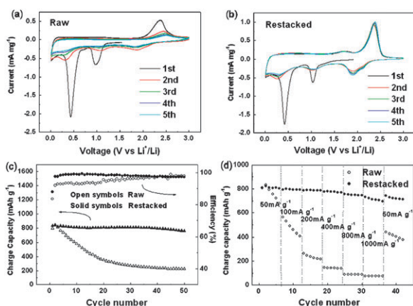
Fig. 3 Electrochemical properties of raw and restacked \text{MoS}_2 : cyclic voltammograms of (a) raw and (b) restacked \text{MoS}_2 at a scanning rate of 0.2 \text{ mV s}^{-1} ; (c) cycling performances at a current density of 50 \text{ mA g}^{-1} ; (d) rate capabilities at different current densities (discharge current density was kept at 50 \text{ mA g}^{-1} ).
