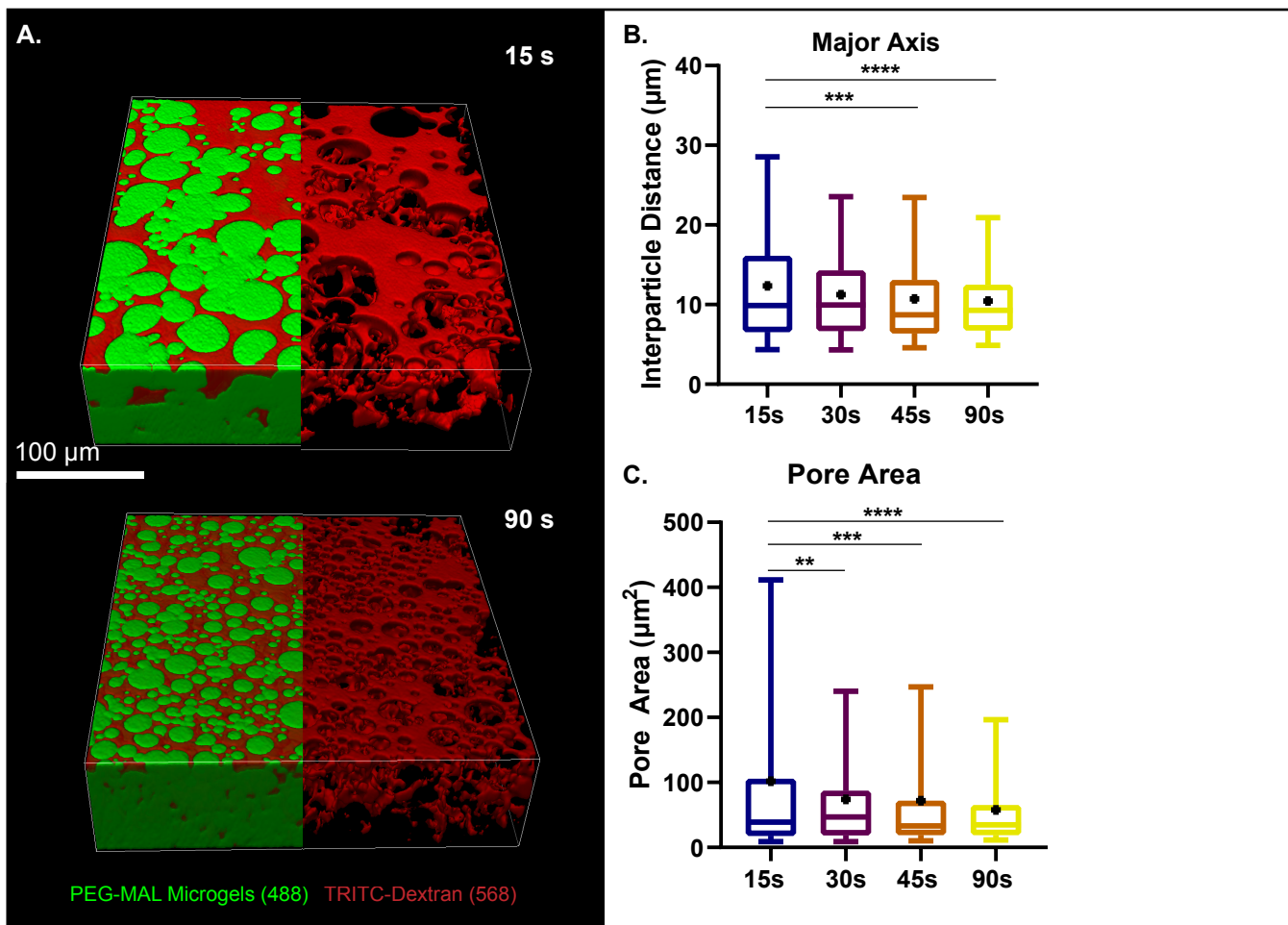
Figure 2: Characterization of microgel diameter and pore size. (A) Z-stack projection of PEG-MAL microgels vortexed for 15 and 90 s. Visualization of void space by using high-molecular-weight TRITC dextran to fill pores within the granular hydrogel scaffold. Scale Bar = 100 \mu\text{m} . (B) Interparticle distance between pores of scaffold at different vortexing times. (C) Pore area analysis at different vortexing times. Data is displayed as a box and whisker plot. The box extends from the 25th to 75th percentile. The median is denoted the middle line. The whiskers extend to the 5th and 95th percentile, mean is denoted by the black dot. Significance determined by one-way ANOVA, P < 0.0001 .
