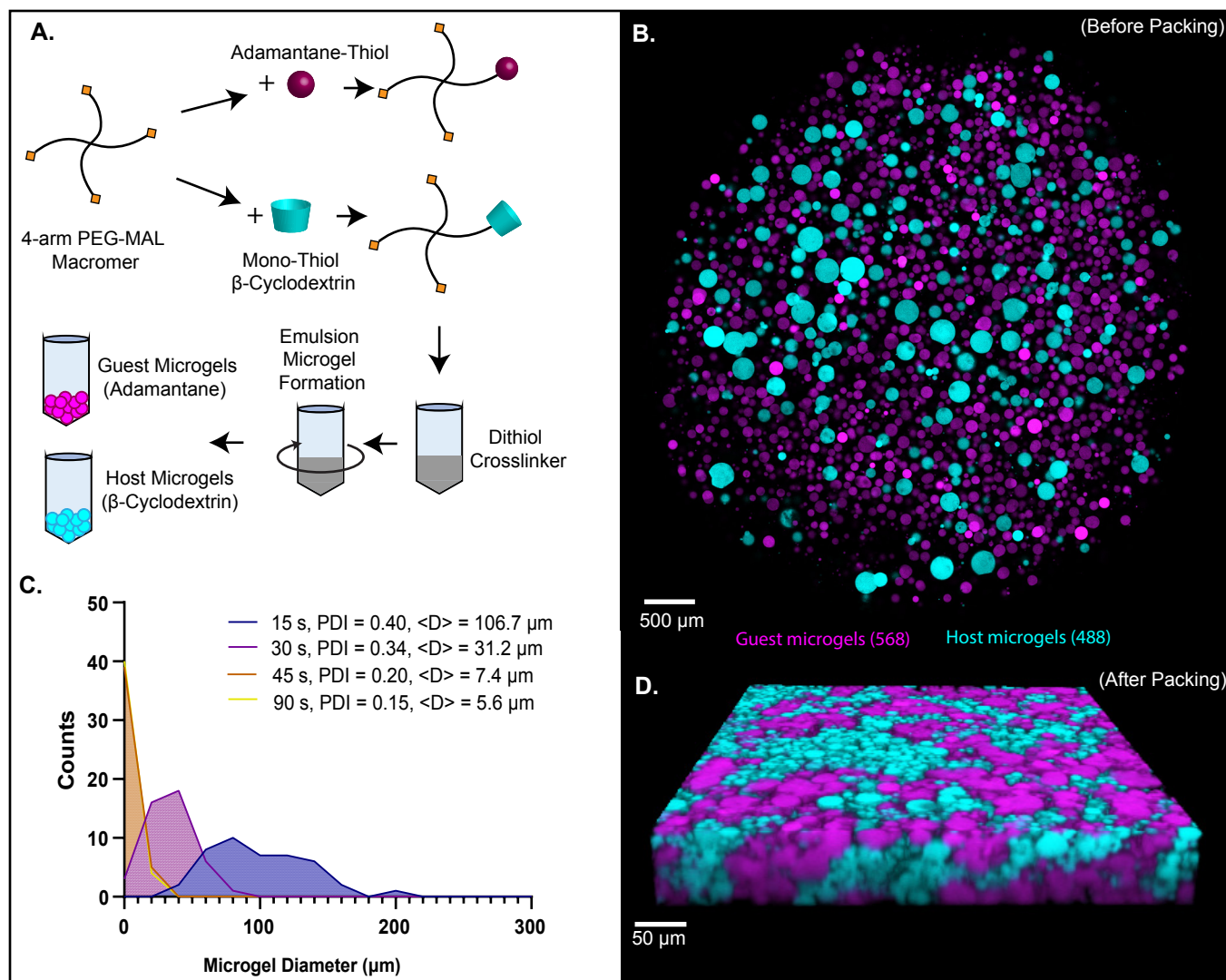
Figure 1: (A) Scheme of PEG-4MAL microgel synthesis. 4-arm PEG-MAL macromer is first functionalized with 1-adamantane-thiol and mono-thiol- \beta -cyclodextrin through Michael-type addition chemistry. Then the PEGylated adamantane (top) and PEGylated \beta -cyclodextrin (bottom) are added to a crosslinker, PEG-dithiol, quickly transferred into mineral oil, and vortexed to create an emulsion. On the right is an example schematic of the two different types of microgels (PEG-A and PEG-B). (B) Confocal image of microgels before packing. (C) Frequency histogram of size distributions of microgels made at 15, 30, 45 and 90 s vortex times. Polydispersity index (PDI) decreased with increasing vortex time. Average diameter, \langle D \rangle , also decreased with increasing vortex time: 106.7 \mu m for 15 s, 31.2 \mu m for 30 s, 7.4 \mu m for 45 s, and 5.6 \mu m for 90 s. (D) Confocal microscopy z-stack volume rendering of packed PEG-A and PEG-B gels. The percolated interstitium is shown between the different species of microgels, allowing for cellular infiltration and uninhibited movement.
