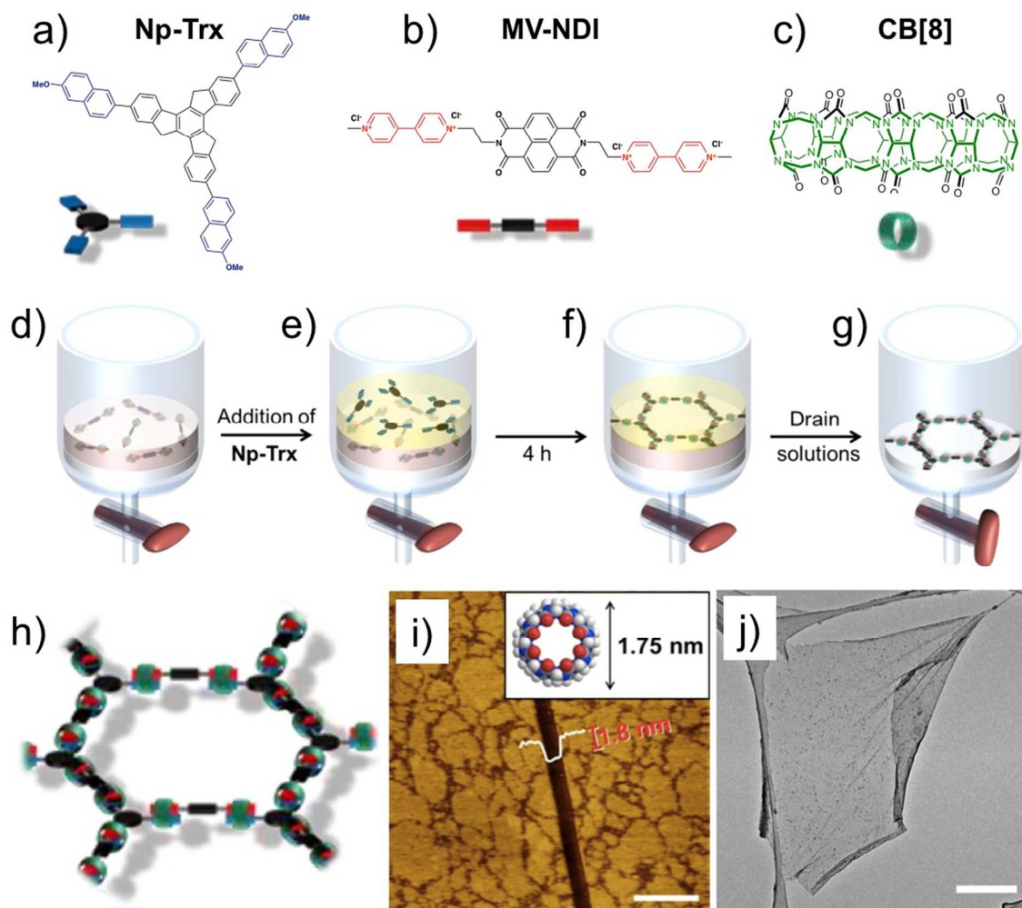
Fig 5. 2D-SOF. (a-c) Molecular structures of the building blocks. (d-e) Schematic showing the process of SOF formation at the liquid-liquid interface. (h) A schematic of the honeycomb SOF (i) AFM image of the 2D-SOF with a scratch with a depth of 1.8 nm. The inset shows the molecular structure of CB[8] with an outer diameter of 1.75 nm, providing evidence for monolayer thickness of the film. The scale bar is 1 \mu\text{m} . (j) TEM-image showing slightly wrinkled, free standing 2D SOF. The scale bar is 2 \mu\text{m} . Reproduced from ref 69 with permission from the American Chemical Society.
