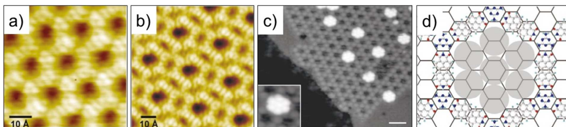
Fig. 1. Early examples of host-guest systems. STM images of the (a) Chicken wire and (b) Flower structure of TMA self-assembled network on HOPG. (c) STM image showing entrapment of heptameric C 60 clusters in the PTCDI-melamine host network assembled on Ag terminated silicon surface. (d) Schematic of the PTCDI-melamine host-guest system. Reproduced from ref. 30 and ref. 31 with permission from Wiley-VCH and Macmillan Publishers. Ltd., respectively.
