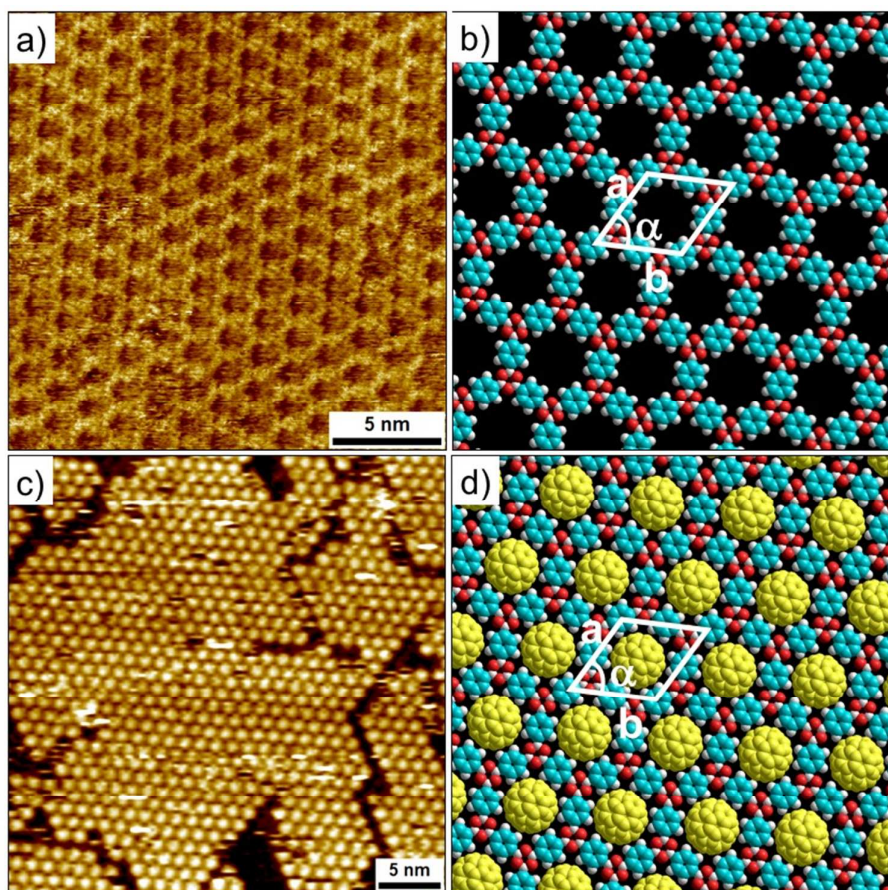
Fig. 16. Host-guest chemistry in covalent organic frameworks. (a) STM image showing the boronic acid COF imaged at the 1-phenyloctane-HOPG interface. (b) Molecular model for the COF. (c) COF- C_{60} host-guest system. (d) Molecular model for the host-guest system. Reproduced from ref. 115 with permission from the Royal Society of Chemistry.
