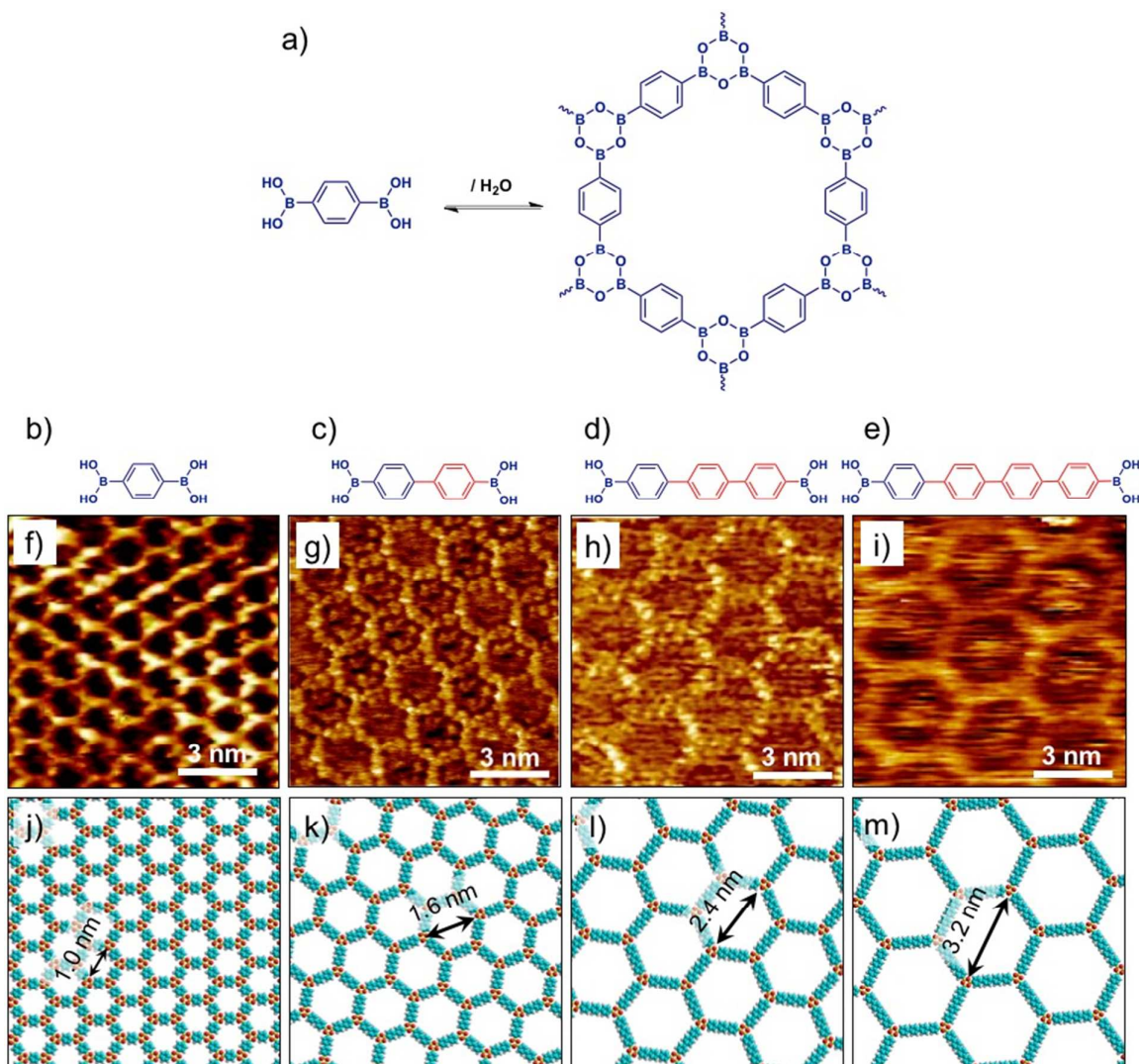
Fig. 6. Surface synthesis of isorecticular 2D-COFs. (a) A reaction scheme showing boronic acid self-condensation to yield boroxine based COF. (b-e) Molecular structures of the boronic acid building blocks with increasing length of the oligophenylene backbone. (f-i) Corresponding STM images of 2D-COF films synthesized on graphite surface (j-m) Molecular models of the isorecticular COF networks. Reproduced from ref 72,73 with permission from the American Chemical Society.
