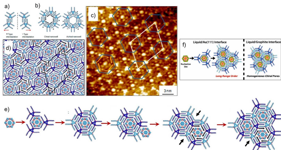
Fig 11 Multicomponent host-guest system obtained using DBA derivatives at the octanoic acid/Au(111) interface. (a, b) Expression of chirality in DBA networks. (c) STM image of the DBA-COR-ISA three component network on Au(111). (d) Molecular model for the DBA-COR-ISA network. (e) Molecular models showing step-by-step growth of the superlattice. The nucleation of the COR-ISA cluster is followed by adsorption of the alkyl chains of three DBA molecules surrounding the cluster. The only way to complete a pore is by the formation of an achiral pore. A COR/ISA cluster is captured in one of the neighboring sites, which leads to formation of either a chiral or an achiral nanowell around it. Assuming formation of a chiral nanowell, the third adjacent nanowell (black arrows) can only adapt an achiral arrangement. The black arrows indicate positions where the structural arrangement of nanowells is predetermined by the combination of structures for the initial two nanowells. (f) A schematic showing the difference in the host-guest patterns obtained on HOPG and Au(111) surface. Reproduced from ref. 17 with permission from the American Chemical Society.
