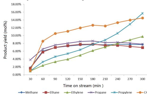
Fig. 10a The evolution of various gas products with time-on-stream over the parent H-ZSM-5 at a temperature of 400 °C, atmosphere pressure
