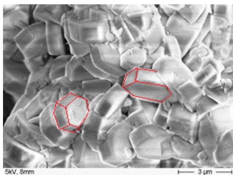
Fig. 7a SEM image of the parent H-ZSM-5
