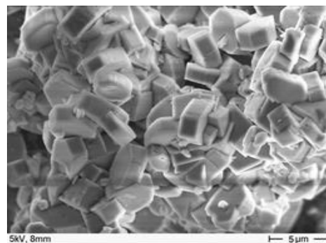
Fig. 7c SEM image of the parent H-ZSM-5 (post reaction)
