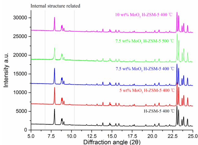
Fig. 2a X-ray Diffraction patterns ( 2\theta = 5 - 25^\circ ) of MoO 3 /ZSM-5 samples with various MoO 3 loadings and prepared at 400 °C/500 °C
