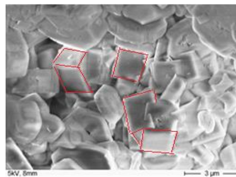
Fig. 7b SEM image of H-ZSM-5 with 7.5wt% MoO 3 - 400 °C
