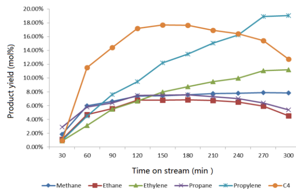
Fig. 10b The evolution of various gas products with time-on-stream over 5wt% MoO 3 /H-ZSM-5 at a temperature of 400 °C, atmosphere pressure
