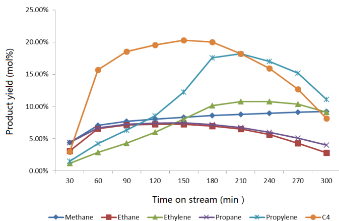
Fig. 10c The evolution of various gas products with time on-stream over 7.5 wt% MoO 3 /H-ZSM-5 at a temperature of 400 °C, atmosphere pressure
