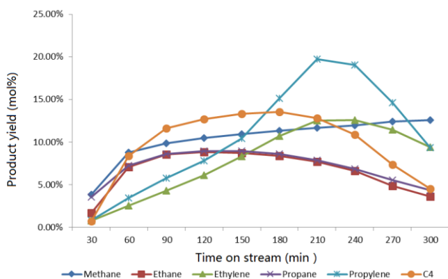
Fig. 10e The evolution of various gas products with time-on-stream over 10 wt% MoO 3 /H-ZSM-5 at a temperature of 500 °C, atmosphere pressure
