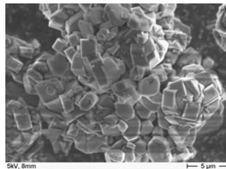
Fig. 7d SEM image of H-ZSM-5 with 7.5wt% MoO 3 - 400 °C (post reaction)
