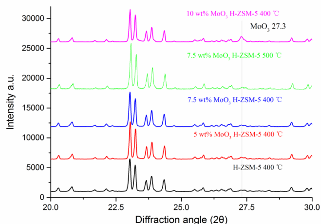
Fig. 2b X-ray Diffraction patterns ( 2\theta = 20 - 30^\circ ) of MoO 3 /ZSM-5 samples with various MoO 3 loadings and prepared at 400 °C/500 °C
