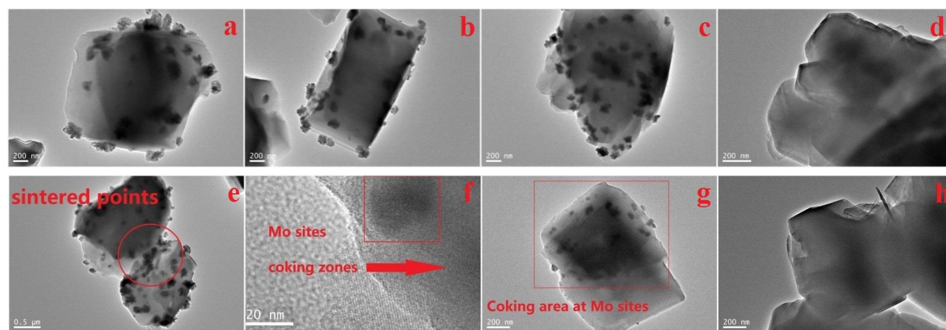
Fig. 8 TEM images of post catalytic-testing samples with different MoO 3 loadings, a , 5wt%, b 7.5 wt%, c 10wt% and d parent H-ZSM-5, e , sintering effects (5wt%), f , amplified coking areas near the Mo species (5wt%), g , coking areas near Mo species (5wt%) and h , parent H-ZSM-5, all the samples are prepared at 400 °C and the MTH reaction proceeded at 400 °C. More images of other samples are included in the Fig.S1-S9.
