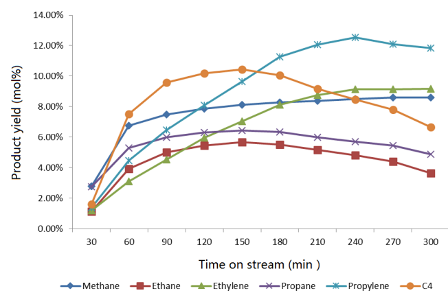
Fig. 10d The evolution of various gas products with time-on-stream over 10 wt% MoO 3 /H-ZSM-5 at a temperature of 400 °C, atmosphere pressure
