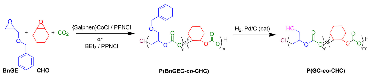
Scheme 2 Terpolymerization of \text{CO}_2/\text{BnGE}/\text{CHO} into P(BnGEC-co-CHC) catalyzed by the \{\text{Salphen}\}\text{CoCl}/\text{PPNCl} or \text{BEt}_3/\text{PPNCl} system, followed by Pd-catalyzed debenzylation resulting into P(GC-co-CHC) terpolymers.
