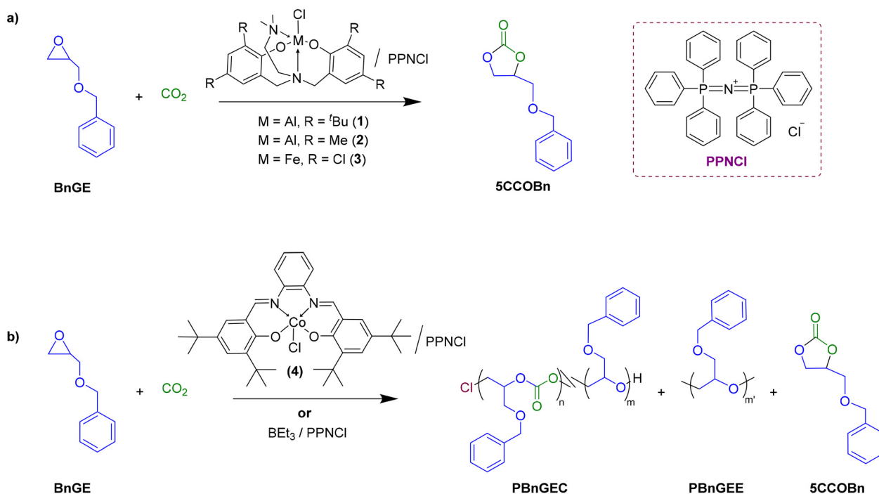
Scheme 1 ROCOP of \text{CO}_2/\text{BnGE} catalyzed by (a) \{\text{ONNO}^{\text{R}2}\}\text{MCl}/\text{PPNCl} (R = t Bu, Me, Cl, M = Al, Fe) complexes resulting in the corresponding five-membered ring benzyloxymethylene cyclic carbonate (5CCOBn), and (b) \{\text{Salphen}\}\text{CoCl}/\text{PPNCl} or \text{BEt}_3/\text{PPNCl} system, resulting in poly(benzyl glycidyl ether carbonate) (PBnGEC), poly(benzyl glycidyl ether) (PBnGEE) and cyclic carbonate (5CCOBn).
