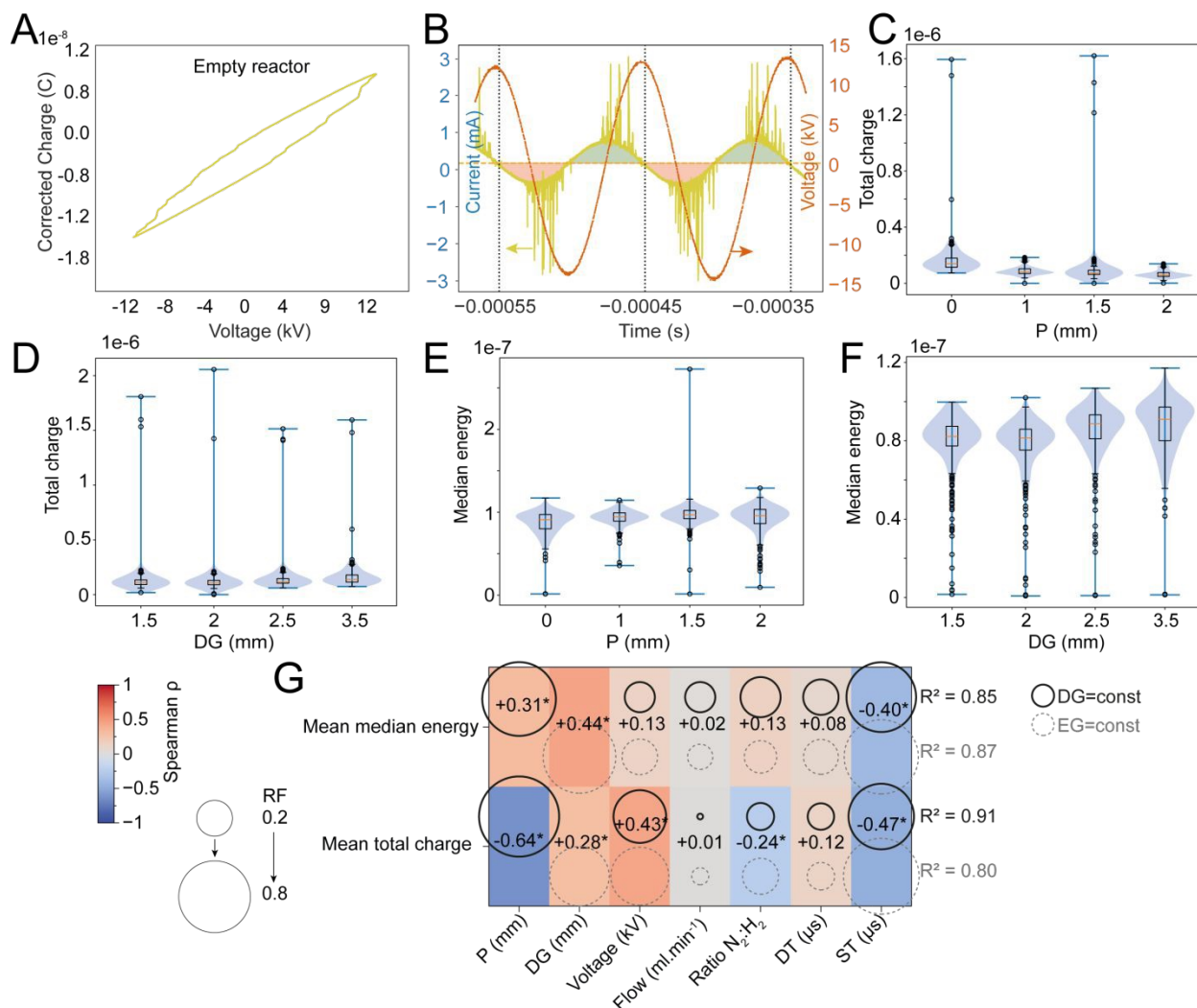
Figure 2. Discharge characteristics as a function of geometry and process settings. (A) Lissajous figure for the empty reactor, showing the capacitor-like charge-voltage relationship across a dielectric layer of MACOR on both the high voltage and ground electrode of 1.2 mm thickness, in an otherwise empty cell. (B) Representative zoomed-in current-voltage waveform of single envelope revealing microdischarge spikes during AC (half-)cycles. (C) Distribution of total charge of microdischarges per one envelope across all experimental conditions at constant DG as a function of dielectric barrier thickness. (D) Distribution of total charge of microdischarges per one envelope across all experimental conditions at constant EG as a function of DG. (E) Distribution of median energy of microdischarges across all experimental conditions at constant DG as a function of dielectric barrier thickness. (F) Distribution of median energy of microdischarges across all experimental conditions at constant EG as a function of DG. (G) Statistical relationships between all geometrical/process inputs and discharge outputs (mean median energy, mean total charge) obtained from Spearman and Random-Forest analyses. The colour indicates the correlation sign and strength (Spearman \rho ); bubble size represents Random-Forest feature importance; numbers to the right denote model R^2 . Asterisks (*) indicate statistically significant correlations ( p < 0.05 , two-tailed Spearman test).
