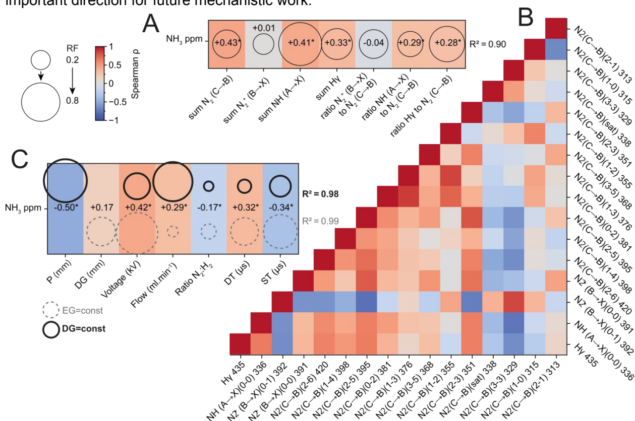
Figure 4. Linking plasma parameters and spectroscopy to ammonia formation. (A) Statistical relationships between OES features and measured NH_3 concentrations. Tile color = Spearman \rho , bubble size = RF importance, R^2 per row indicates predictive power. The strong contributions of N_2^+(B-X) and NH(A-X) emissions demonstrate that excitation
