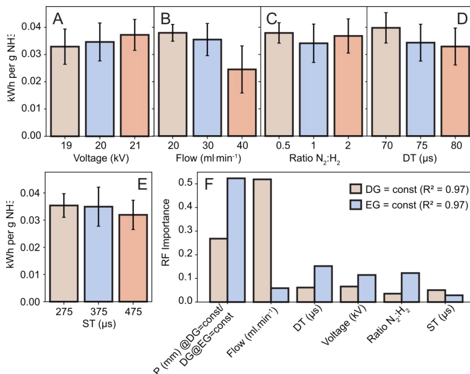
Figure 5. Energy-efficiency analysis of plasma ammonia synthesis. (A–E) Experimental mean \pm standard-deviation plots of \text{NH}_3 production efficiency ( \text{kWh g NH}_3^{-1} ) versus each varied input: applied voltage, gas-flow rate, \text{N}_2:\text{H}_2 ratio, DT, and ST. (F) Random-Forest summary of feature importance for predicting energy efficiency from all input variables. Efficiency improves primarily with optimized gas flow and applied voltage, while timing parameters (DT/ST) and pellet geometry play secondary roles.
