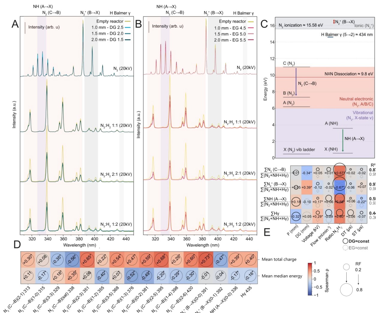
Figure 3. Optical-emission spectroscopy (OES) signatures and their statistical interpretation. (A, B) Representative emission spectra for (A) constant EG, and (B) constant DG under different gas mixtures ( N_2:H_2 = 1:1, 2:1, 1:2 ) for different pellet thicknesses P, and for the empty reactor, with reference spectra for pure N_2 . (C) Schematic of the electronic and vibrational energy levels of N_2(C-B) , N_2^+(B-X) , NH(A-X), and H (Balmer) transitions probed by OES, also indicated in (A, B). (D) Spearman correlations between discharge-derived quantities (mean total charge, mean median energy) and the intensity of each individual spectral line obtained via Gaussian integration (see Supplementary Table S2 for more details), revealing which discharge properties most strongly influence which excited-state populations. Tile color encodes Spearman \rho . (E) Combined analysis of geometrical/process inputs versus summed integrated OES band intensities ( N_2(C-B) , N_2^+(B-X) , NH(A-X), H Balmer). Bubble size indicates the Random-Forest importance, and right-hand labels the model R^2 . The figure highlights how voltage and gas composition jointly govern excitation of nitrogen and hydrogen species.
