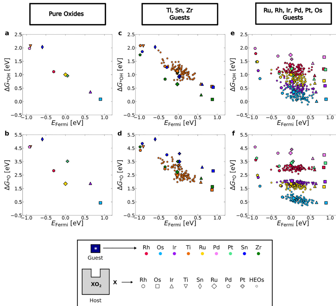
Fig. 2 Correlation between adsorption energies of the \ast\text{OH} and \ast\text{O} intermediates and the E_{\text{Fermi}} of the bare surface slabs for the pure oxides (a) and (b), the Zr, Ti, and Sn guests data (c) and (d), the Ru, Rh, Os, Ir, Pd, and Pt guests data (e) and (f). Markers represent different host compositions and colours correspond to different guest elements, as described in the legend.
