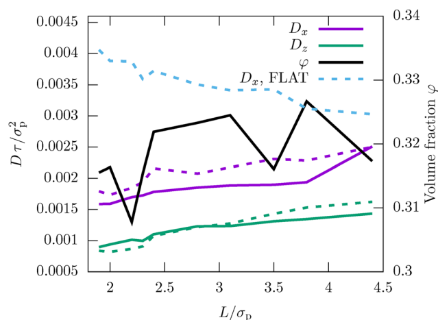
Fig. 2 Diffusion coefficient D along the in-plane (x) and the lateral (z) direction for different confinement lengths L . The diffusion coefficient was extracted from the data in Fig. 1 using linear fits. The diffusion coefficient is compared to the volume fraction \phi .
