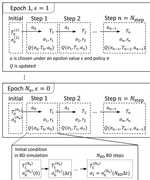
Fig. 2 Schematic of Q-learning at each epoch with the \epsilon -greedy method. The action a is chosen based on the current policy \pi and \epsilon . Q is updated according to eqn (S2) (ESI†). The Brownian dynamics (BD) simulation is conducted for every action step in N_{\text{step}} of each epoch.
