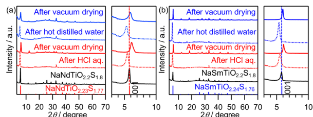
Fig. 6 XRD patterns of the sulfurized products, \text{NaMTiO}_{2.2}\text{S}_{1.8} ( M = (a) Nd, (b) Sm) and the samples after stirring under dark conditions in an HCl aqueous solution for 24 h or hot distilled water for 72 h, followed by vacuum drying, along with the reference patterns of \text{NaNdTiO}_{2.23}\text{S}_{1.77} (this work) and \text{NaSmTiO}_{2.24}\text{S}_{1.76} (this work).
