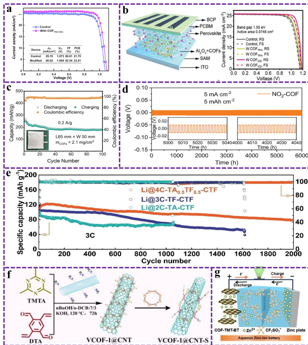
Fig. 17 (a) J - V characteristics of the PSCs without and with COFTPA-TZDA under standard illumination conditions. Reproduced from ref. 88 with permission from CCS Chemistry, copyright 2024. (b) Device structure of the inverted PSC and J - V curves of the COF-modulated inverted PSC devices. Reproduced from ref. 271 with permission from John Wiley and Sons, copyright 2024. (c) Cycling performance of the pouch cell at 0.2 A g -1 for 100 cycles. Reproduced from ref. 272 with permission from John Wiley and Sons, copyright 2024. (d) Galvanostatic cycling of Li-NO 2 -COF symmetric cells at a current density of 5 mA cm -2 . Reproduced from ref. 274 with permission from John Wiley and Sons, copyright 2023. (e) Long-term cycles of full cells based on Li@2C-TA-CTF, Li@3C-TF-CTF, and Li@4C-TA 0.5 TF 0.5 -CTF at 3C. Reproduced from ref. 134 with permission from John Wiley and Sons, copyright 2024. (f) Schematic illustration of the synthesis of VCOF-1@CNT and the inverse vulcanization of VCOF-1@CNT with elemental sulfur. Reproduced from ref. 275 with permission from Elsevier, copyright 2024. (g) Schematic of the COF-TMT-BT||Zn(CF 3 SO 3 ) 2 ||Zn energy storage system. Reproduced from ref. 278 with permission from John Wiley and Sons, copyright 2023.
