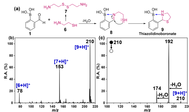
Fig. 4 (a) Formation of thiazolidinoboronate (9) via iminoboronate (8) in electrospayed microdroplets. (b) Positive mode nESI mass spectrum showing the product of the reaction between cysteamine and 2-FPBA in ACN microdroplets. Structures are shown for the labeled peaks. (c) MS/MS spectrum of the mass-selected thiazolidinoboronate product, [9+H] + , m/z 210, recorded using collision-induced dissociation (CID).
