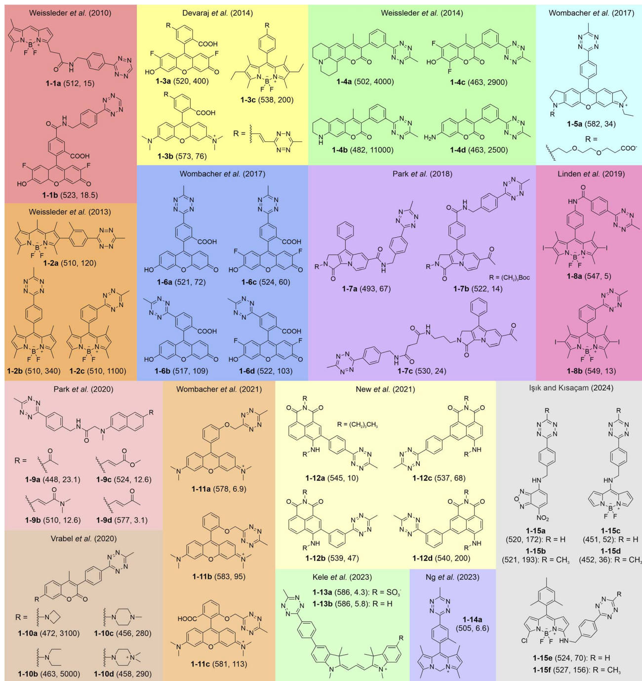
Fig. 1 Representative molecular structures of tetrazine-isolated fluorogenic labels with visible fluorescence. The numbers in each bracket show the \lambda_{\text{em}} (nm) and FE ratios (-fold), respectively. The reaction conditions are listed in Table S1, ESI.†
