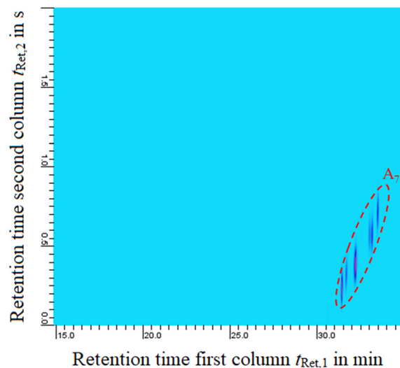
Fig. 7 GC × GC-FID chromatogram of fresh DBT as delivered by the manufacturer.
