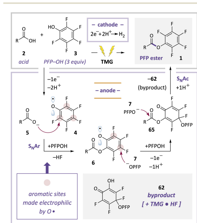
Fig. 7 Revised mechanistic hypothesis. Deprotonation and anodic oxidation of PFP-OH ( 3 ) generates oxyl radical 4 , which undergoes S N Ar with carboxylate 5 . Resulting open-shell O-aryl ester 6 is oxidized further and trapped by a second equivalent of PFP-O - ( 7 ), producing acyl electrophile 65 . S N Ac by a third equivalent of PFP-O - ( 7 ) affords PFP ester 1 and byproduct 62 .
