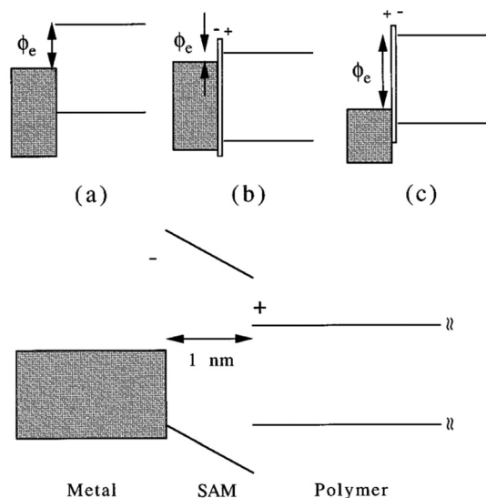
Fig. 5 Schematic energy level diagrams of metal/organic interfaces: panel a, untreated interface; panel b and panel c, dipole layer which decreases and increases the electron Schottky energy barrier, respectively; and panel d, magnified view of the interface. Reproduced from ref. 79 with permission from American Physical Society, copyright 1996.
