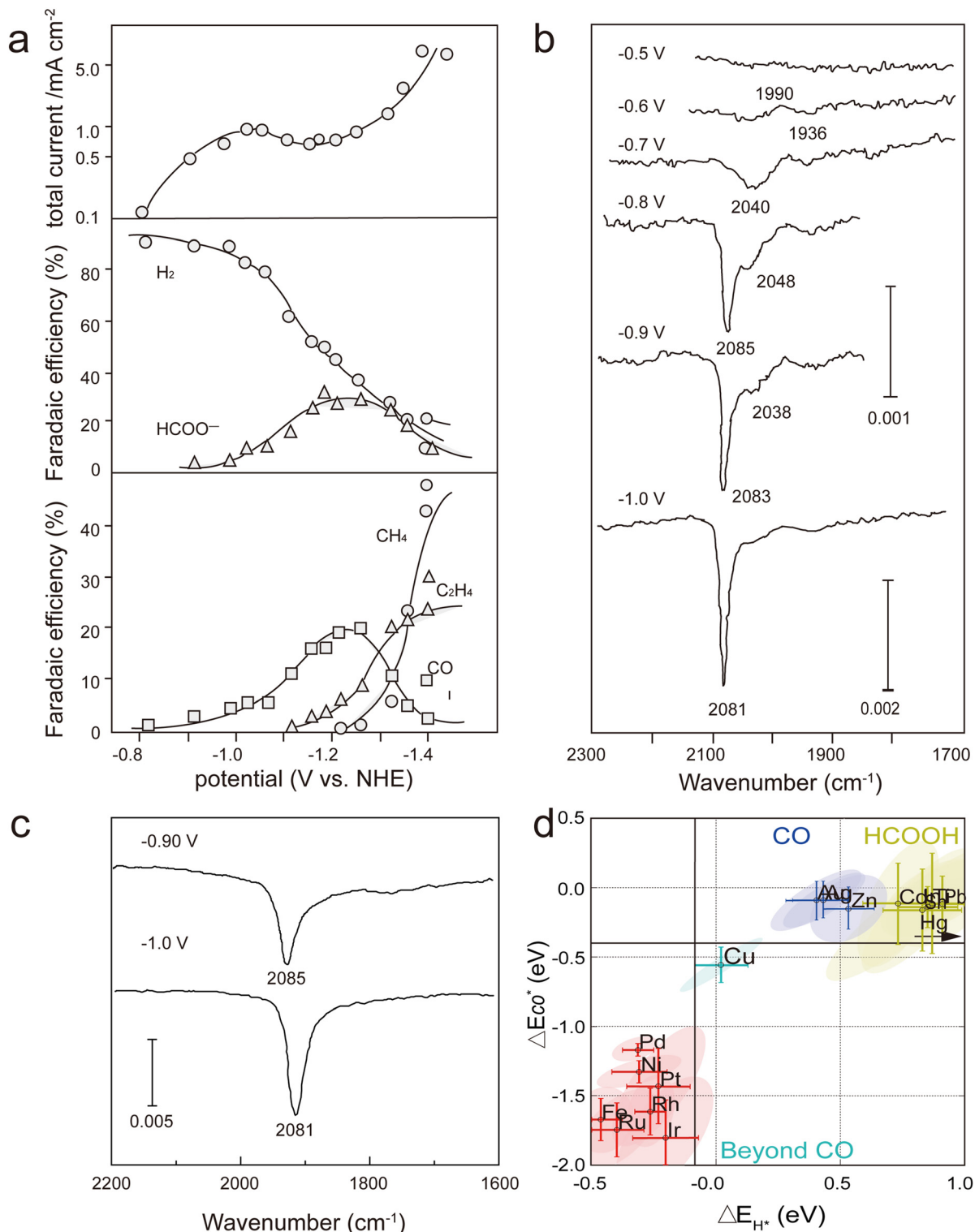
Fig. 1 (a) FE variations of \text{CO}_2 reduction products in 0.1 M \text{KHCO}_3 at 19 ^\circ\text{C} . (b) In situ IR spectra of adsorbed species on Cu during CO electroreduction at different potentials in 0.2 M \text{KHCO}_3 . (c) In situ IR spectra of adsorbed species on Cu during \text{CO}_2 electroreduction at different potentials in 0.1 M \text{KHCO}_3 . (d) \text{CO} and \text{H} binding energies set Cu apart from other metals. (a) Reprinted with permission from Hori et al. 52 Copyright 1989, the Royal Society of Chemistry. (b and c) Reprinted with permission from Hori et al. 56 Copyright 1995, Elsevier. (d) Reprinted with permission from Baggett et al. 60 Copyright 2017, John Wiley and Sons.
