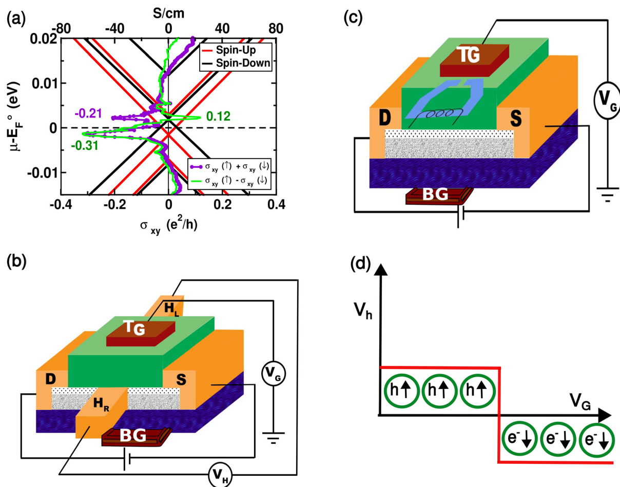
Fig. 3 (a) Anomalous Hall charge conductivity ( \sigma_{xy}^{\uparrow} + \sigma_{xy}^{\downarrow} ) and anomalous Hall spin conductivity ( \sigma_{xy}^{\uparrow} - \sigma_{xy}^{\downarrow} ), \sigma_{xy} , as a function of Fermi energy ( E_F ) of the half-electron doped gated graphene/1T-CrTe 2 heterostructure, obtained using Wannier functions and 500 \times 500 k -points. Peaks arise as the E_F crosses Dirac points giving charge and spin currents. A schematic model of the Anomalous Hall Transistor (AHT) that stores binary information through ( V_G )-switchable Hall signals that can be read with electric voltage (b) or with a magnetic head (c). This is possible because ( V_G ) switches both charge and spin that cause the anomalous Hall effect (d).
