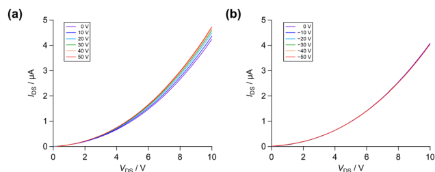
Fig. 5 FET characteristics of \text{C}_{60} nanowires. I - V characteristics ( I_{\text{DS}} vs. V_{\text{DS}} ) at (a) V_{\text{G}} = 0 to 50 V and (b) V_{\text{G}} = 0 to -50 V in a step of 10 V. These measurements were fixed for W = 1500 \text{ }\mu\text{m} and f = 1 \times 10^{11} \text{ cm}^{-2} .
