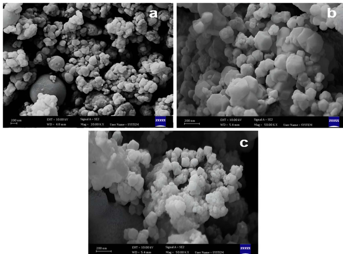
Fig. 7 SEM images of (a) \text{Fe}_3\text{O}_4@MCM-41 , (b) UiO-66-NH_2 , and (c) \text{Fe}_3\text{O}_4@MCM-41@UiO-66/SB-Pd .
