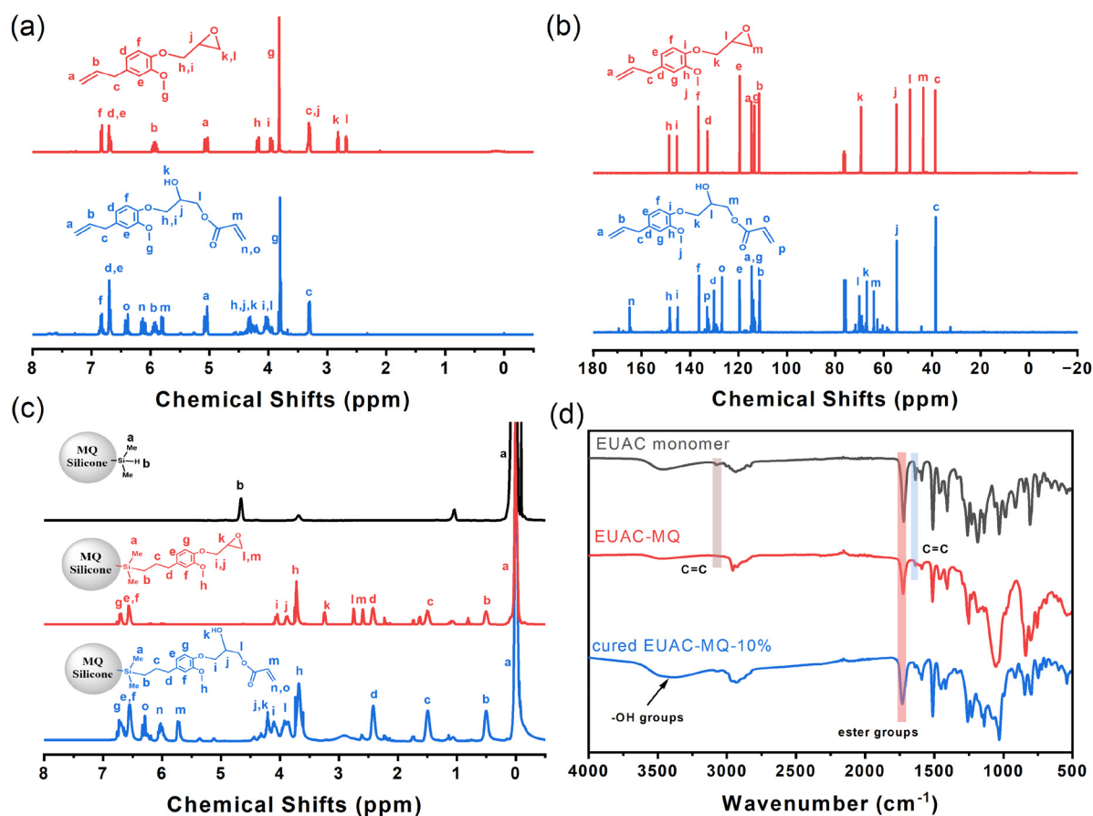
Fig. 3 NMR spectra of EUPEP and EUAC: (a) 1 H NMR; (b) 13 C NMR; and (c) 1 H NMR spectra of EUAC-MQ; and (d) FT-IR spectra of EUAC, EUAC, and EUAC-MQ-10%.
