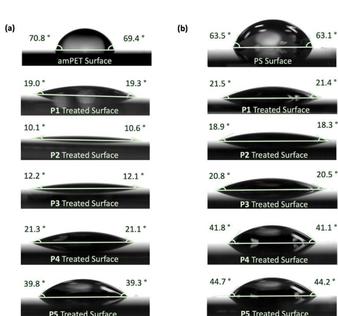
Figure 6: Contact angle measurements of a 5 \mu\text{L} droplet of deionised water on a (a) amPET surface and 1% (w/w) SRP-treated amPET surface; (b) PS surface and 1% (w/w) SRP-treated PS surface; after dip rinsing in \text{H}_2\text{O} .
