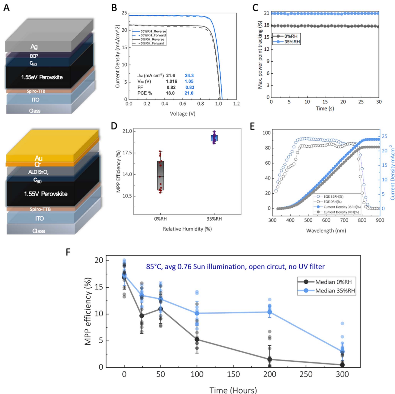
Fig. 4 (A) fully vacuum deposited device stack using BCP/Silver or ALD \text{SnO}_2/\text{Cr}/\text{Au} for standard solar cells and stable contacts used for stability analysis, respectively. (B) J/V curves of devices fabricated where annealing is done in presence of 0% RH (nitrogen) and 35% RH. (C) Maximum power point tracking of champion devices obtained from nitrogen (0% RH) and 35% RH annealing, respectively. (D) Statistical comparison of max power point efficiency obtained from maximum point tracking. (E) External quantum efficiency of a device where the perovskite is annealed under 0% RH and 35% RH. (F) Maximum power point efficiency as a function of time for cells aged under open-circuit at elevated temperature under light (85 °C, 0.76 suns illumination from a xenon lamp aging box with no UV filter) ~ISOS-L-2, where the perovskite was annealed under 0% RH in nitrogen and 35% RH in air. The cells were occasionally removed from the ageing rig, allowed to cool to room temperature, and measured under AM1.5100 \text{mW cm}^{-2} simulated sun light to determine the photovoltaic performance parameters, including the mpp efficiency. The error bars represent the median standard deviation.
