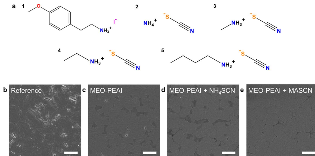
Fig. 1 (a), Molecular structures of 4-methoxy-phenylethylammonium iodide (MEO-PEAI), ammonium thiocyanate (NH 4 SCN), methylammonium thiocyanate (MASCN), ethylammonium thiocyanate (EASCN) and n -butylammonium thiocyanate (BASCN), respectively (1–5). (b–e) Scanning electron microscopy (SEM) images of buried interface of reference, MEO-PEAI, MEO-PEAI + NH 4 SCN and MEO-PEAI + MASCN treated perovskite films. Scale bars, 1 μm.
