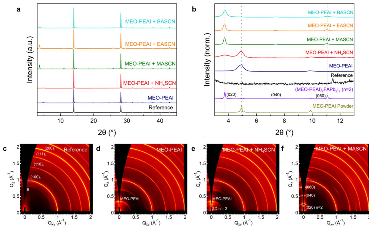
Fig. 2 (a) X-ray diffraction (XRD) patterns of perovskite films. (b) Enlarged XRD pattern in the 2θ range between 3° and 12° of perovskite films. (c–f) Two-dimensional grazing-incidence wide-angle X-ray scattering (GIWAXS) patterns of reference, MEO-PEAI, MEO-PEAI + NH 4 SCN, MEO-PEAI + MASCN treated perovskite films.
