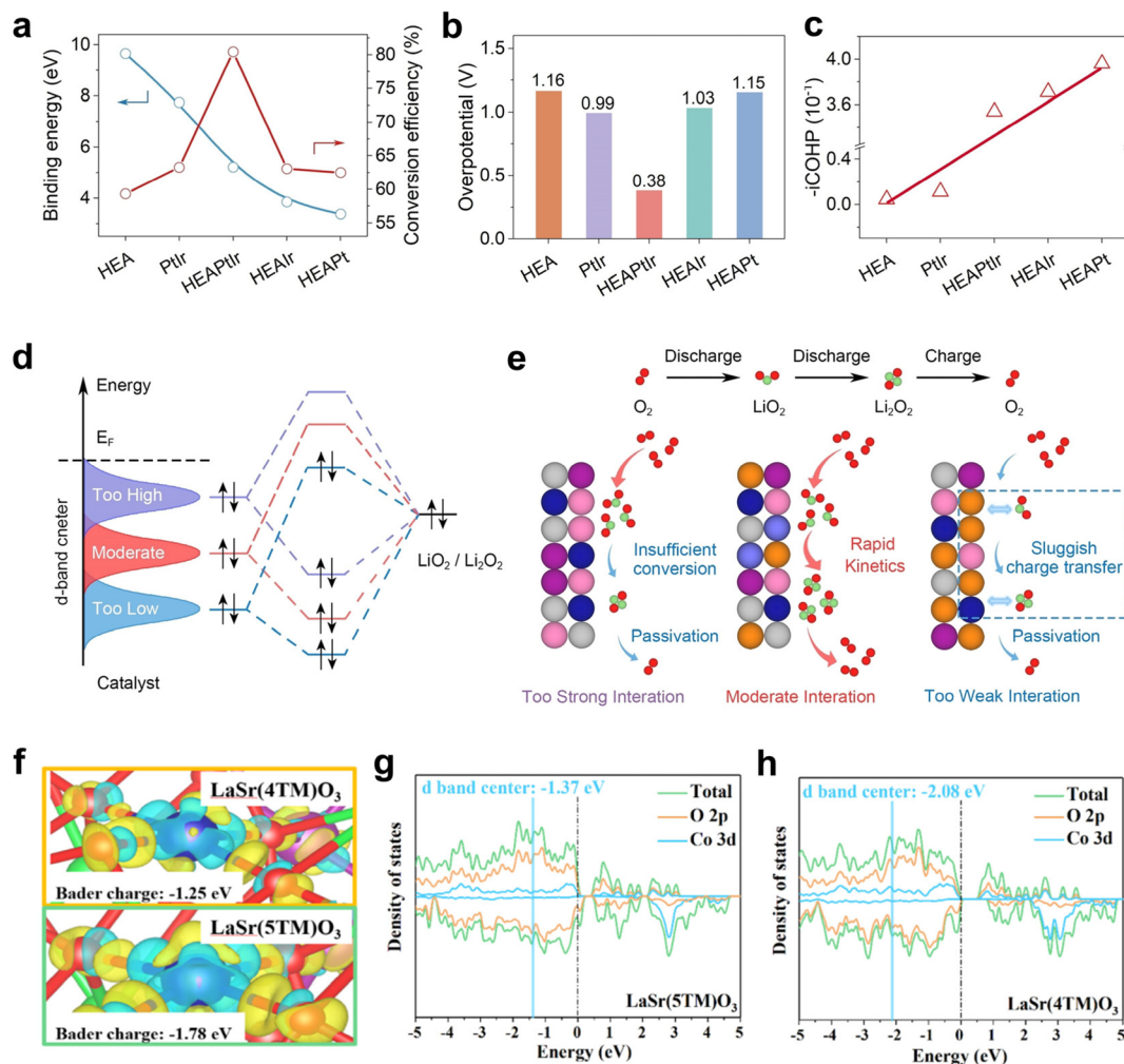
Fig. 8 (a) Binding energy of LiO 2 with cathode catalysts (HEA, PtIr, HEAPtIr, HEAIr, HEAPt) and the corresponding energy conversion efficiency. (b) Overpotentials of different alloy catalysts at a current density of 500 mA h g -1 . (c) -iCOHP values of the corresponding systems. (d) Orbital interactions between different d-band center catalysts and LiO 2 /Li 2 O 2 . (e) Corresponding catalytic effects. 116 (f) Charge density differences at Co sites in LaSr(5TM)O 3 and LaSr(4TM)O 3 (yellow regions represent charge accumulation, and blue regions represent charge depletion). PDOS and DOS of (g) LaSr(5TM)O 3 and (h) LaSr(4TM)O 3 . 81
