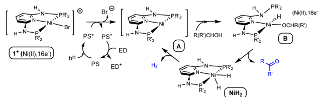
Scheme 4 Proposed mechanism for the photocatalytic molecular acceptorless dehydrogenation of alcohols with [Ni(2,6-(Ph 2 PNH) 2 (NC 5 H 3 ))Br] + . PS = Ru(bpy) 3 3+ , ED = DMEA.
