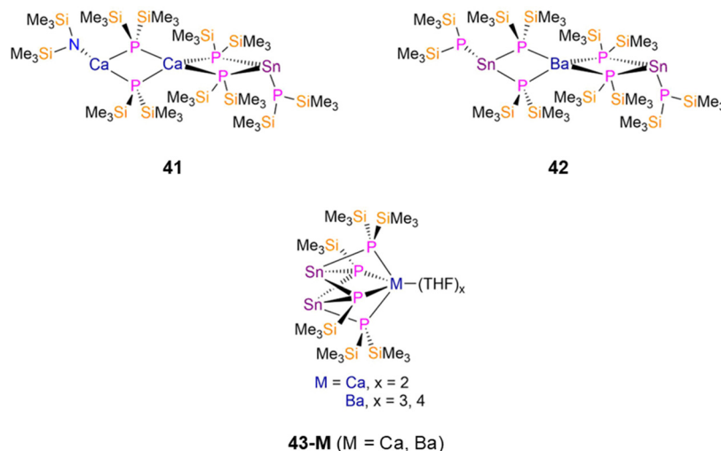
Fig. 12 Heterometallic group 14 P'' complexes [Sn(P'')(μ-P'')_2Ca(μ-P'')_2Ca(N'')] ( 41 ), [{Sn(P'')(μ_2-P'')}_2Ba] ( 42 ), [M(THF)_x\{Sn(μ_2-P'')\}_2\{Sn(μ_3-P'')\}_2] ( 43-M ; M = Ca, x = 2, M = Ba, x = 3, 4, P'' = \{P(SiMe_3)\} ).
