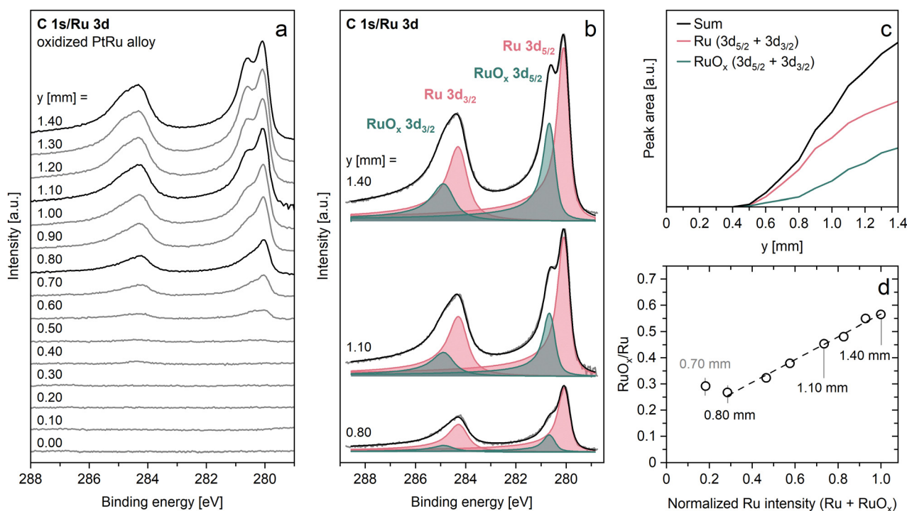
Fig. 4 (a) C 1s/Ru 3d y scan of the PtRu near-surface alloy after exposure to O 2 at 600 K ( y = 0.00 mm \rightarrow 1.40 mm, in 0.10 mm steps). (b) Selected C 1s/Ru 3d spectra at y = 1.40, 1.10 , and 0.80 mm to illustrate the applied fit model. (c) Corresponding quantitative plot of the peak areas against the measurement position. (d) Plot of the relative oxide amount, \text{RuO}_x/\text{Ru} , as a function of the combined normalized Ru intensity ( \text{Ru } 3d + \text{RuO}_x ).
