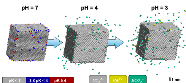
Fig. 2 Snapshots of the calcite crystallite as obtained from MD simulations in aqueous solution (not shown) at various pH values. Left: Calcite crystal at pH = 7. A color code is used to indicate local differences in proton affinity. Center and right: Same model, but after 1 ns propagation at pH = 4 and pH = 3, respectively. While the (notched) calcite crystallites are illustrated by the corresponding molecular surface (grey), HCO_3^- and Ca^{2+} ions that are released at are indicated in green and yellow, respectively. For comparison, the calcium ions that are released at pH = 3 are also highlighted in yellow color for the crystallite model referring to pH = 7. Note that these 'loose' Ca^{2+} species are predominantly located at the crystallite corners and edges, respectively. No CO_3^{2-} ions were released in any of our simulation runs.
