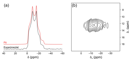
Fig. 2 (a) 23 Na (14.1 T, 16 kHz MAS) MAS NMR spectrum of Na 2 ADC(MW) (black line) and line shape simulated using parameters determined by analytical fitting (see Table S4 in the ESI † ). (b) 23 Na (14.1 T, 16 kHz MAS) MQMAS spectrum of Na 2 ADC(MW) acquired using an amplitude-modulated z-filter pulse sequence and shown after shearing.
