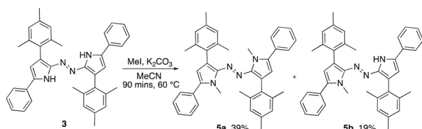
Scheme 2 Synthesis of methylated azobispyrroles.
