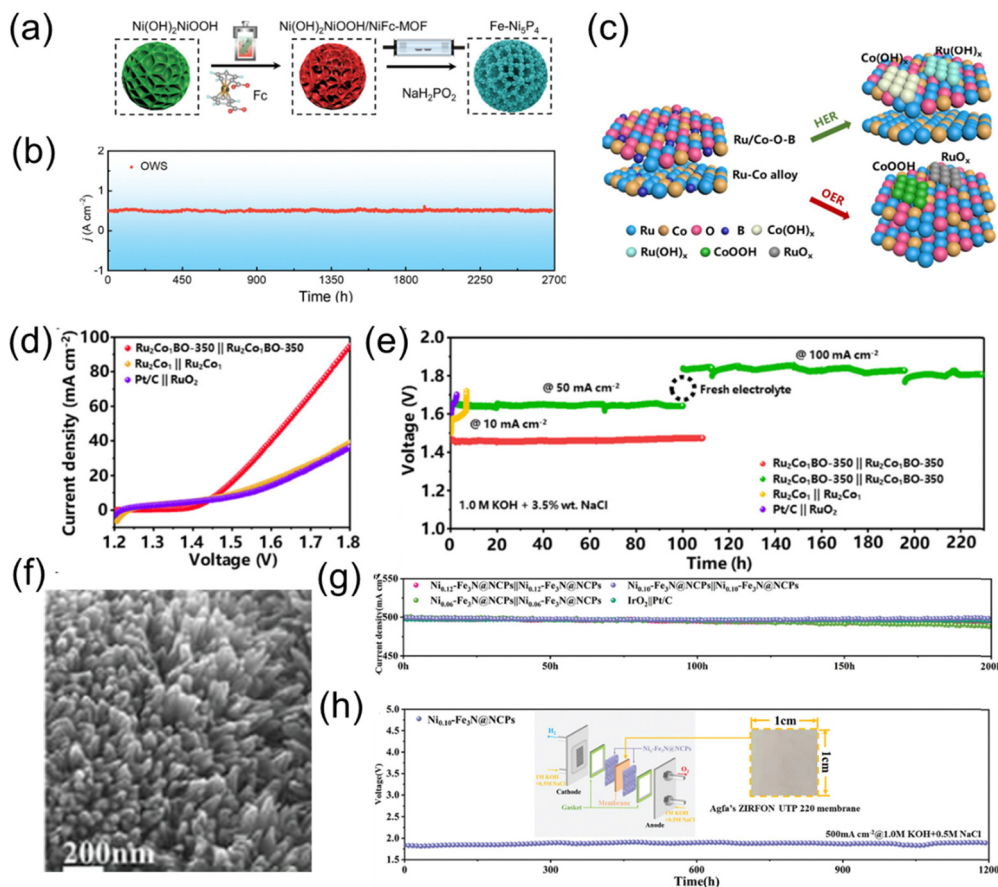
Fig. 2 (a) Schematic illustration of the synthesis process of Fe-Ni 5 P 4 . (b) Chronoamperometry curve of Fe-Ni 5 P 4 || Fe-Ni 5 P 4 toward OWS at 500 mA cm -2 . 27 Copyright © 2024 Wiley-VCH GmbH. (c) Schematic illustration of the Ru 2 Co 1 BO-350 surface reconstructed in the HER and OER. (d) Polarization curves. (e) Long-term stability at current densities of 10, 50, and 100 mA cm -2 . 28 Copyright © 2023, American Chemical Society. (f) SEM images of Ni 0.10 -Fe 3 N@NCPs. (g) Time-dependent current density curves of Ni x -Fe 3 N@NCPs || Ni x -Fe 3 N@NCPs and IrO 2 || Pt/C. (h) Voltage profile of zero-gap commercial electrolyzer with time at current densities of 500 mA cm -2 . 29 Copyright © 2024 Wiley-VCH GmbH.
