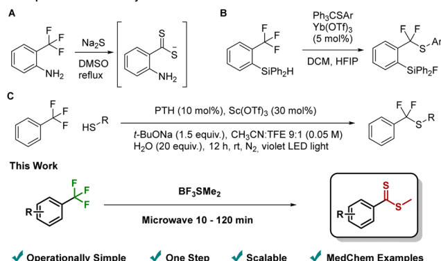
Fig. 1 Top: Examples of \text{CF}_3 /sulfur transformations: (A) sulfur insertion into activated \text{CF}_3 -group 3a , (B) substrate assisted C–F activation 3b , (C) Lewis acid promoted, photo-redox catalyzed C–F activation. 3c Bottom: This work.
