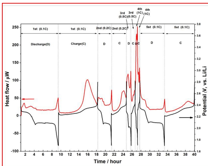
Fig. 16 Discharge profile (black) and heat generation (red) at different C-rates (0.1 C to 1 C) for a nitrogen and phosphorus doped carbon-sulfur cathode. Reproduced with permission from ref. 98, Copyright (2023) Royal Society of Chemistry.
