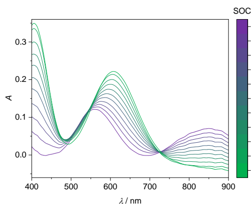
Fig. 4 UV-Vis absorption spectra of the V(II)/V(III) half-cell for wavelengths between 400 and 900 nm depending on the SOC at 298.15 K. Bold lines: spectra of single vanadium species, V(II) (purple) and V(III) (green). Thin lines: spectra at different SOC as indicated by the color bar, corresponding to mixtures of V(II) and V(III). The solution comprises 1.774 \text{ mol kg}^{-1} vanadium in aqueous solution with 4.384 \text{ mol kg}^{-1} sulfuric acid.
