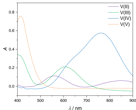
Fig. 3 UV-Vis absorption spectra for wavelengths between 400 and 900 nm of 1.774 \text{ mol kg}^{-1} vanadium in different oxidation states in aqueous solution with 4.384 \text{ mol kg}^{-1} sulfuric acid at 298.15 K.
