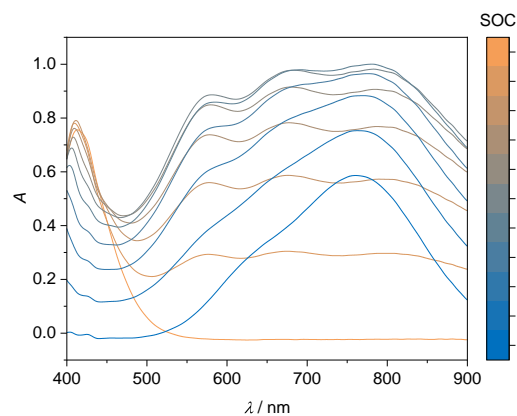
Fig. 5 UV-Vis absorption spectra of the V(V)/V(IV) half-cell for wavelengths between 400 and 900 nm depending on the SOC at 298.15 K. Bold lines: spectra of single vanadium species, V(V) (orange) and V(IV) (blue). Thin lines: spectra at different SOC as indicated by the color bar, corresponding to mixtures of V(V) and V(IV). The solution comprises 1.774 \text{ mol kg}^{-1} vanadium in aqueous solution with 4.384 \text{ mol kg}^{-1} sulfuric acid.
