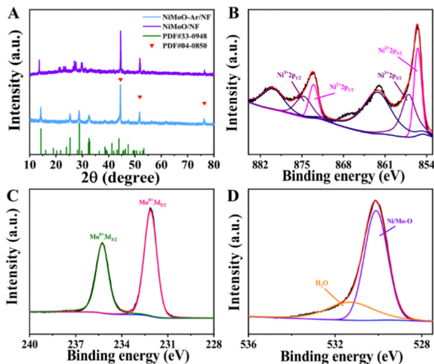
Fig. 2 (A) XRD patterns of NiMoO-Ar/NF and NiMoO/NF. (B) Ni 2p spectra. (C) Mo 3d spectra. (D) O 1s spectra.
