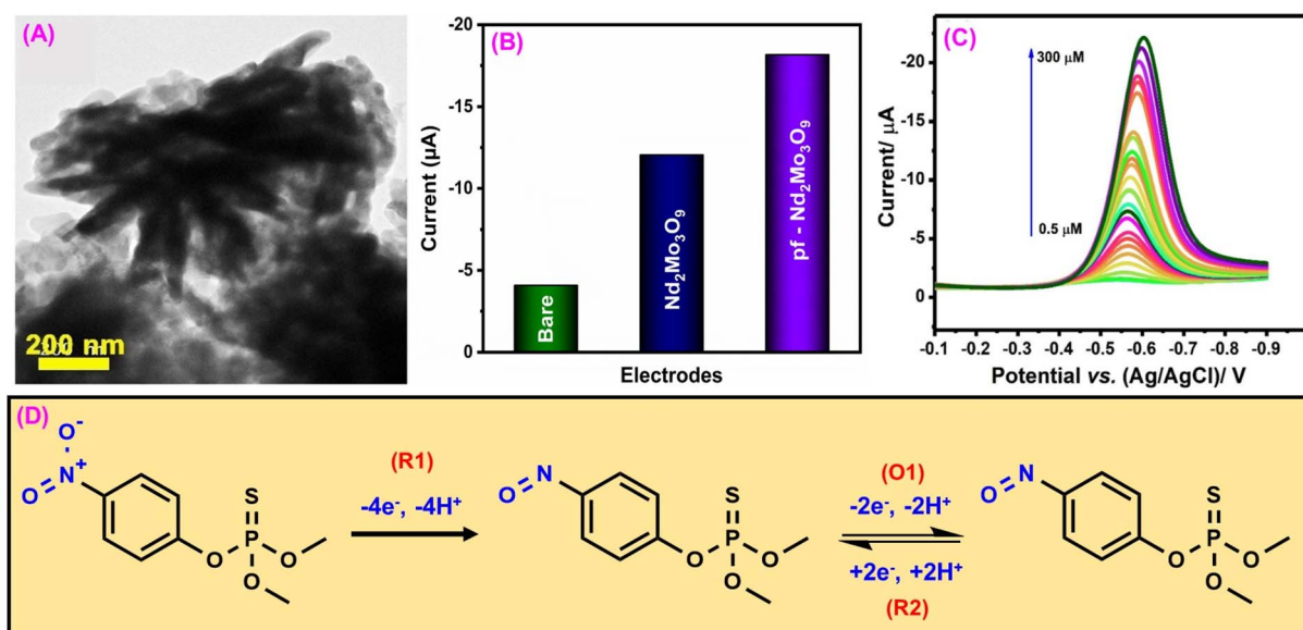
Fig. 2 (A) TEM image of pf-Nd 2 Mo 3 O 9 . (B) CV investigation of the bare GCE (green), Nd 2 Mo 3 O 9 (blue), and pf-Nd 2 Mo 3 O 9 (purple). (C) DPV signal of pf-Nd 2 Mo 3 O 9 for MPN detection. (D) Electrochemical detection mechanism of MPN 103 (modified). ((A and C) License number: 5542351439158).
