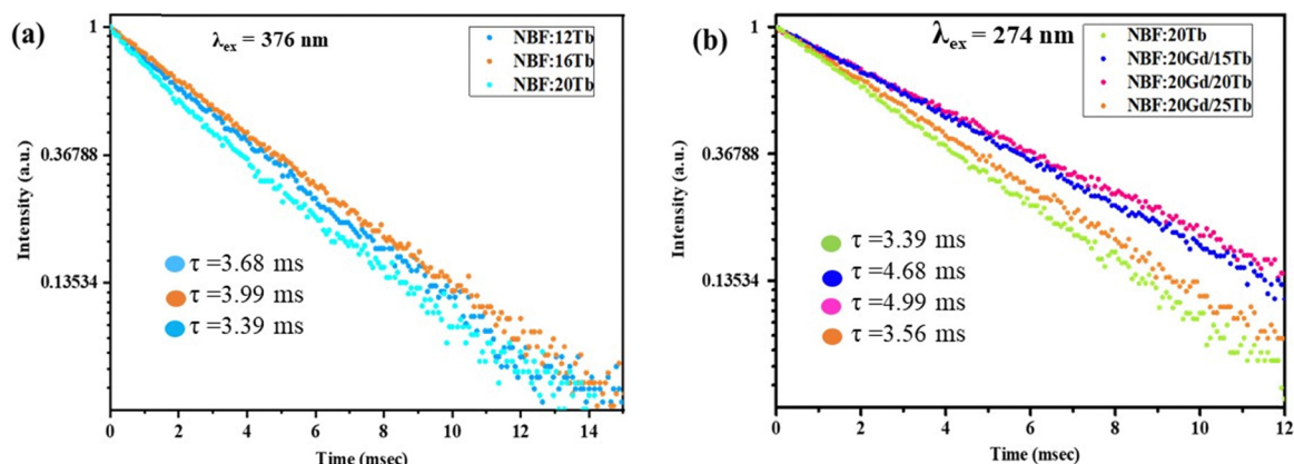
Fig. 5 (a) PL decay curves of NBF:xTb and (b) NBF:20Gd,xTb ( x = 15, 20, 25 ) nanoparticles.
