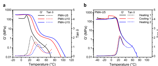
Fig. 8 DMTA curves of the PMA-UPy networks. (a) Storage modulus ( G' ) and loss factor ( \tan \delta ) as a function of temperature for all polymers; (b) storage modulus ( G' ) and \tan \delta as a function of temperature for a second sample of PMA-U5 in two heating runs and one cooling run. Note that the absolute G' values are lower than expected for glassy polymers indicating that the calibration was not optimal, which will, however, not influence the relative trends.
