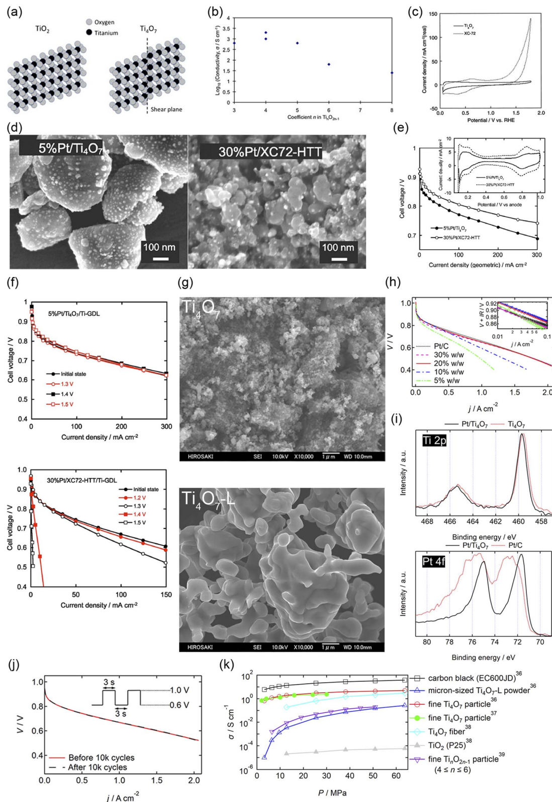
Fig. 4 (a) Crystal structure of rutile TiO 2 and Ti 4 O 7 . (b) A conductivity versus n in Magnéli-phase Ti 4 O 2n-1 curve. Reproduced with permission. 33 Copyright 2010, Elsevier. (c) Cyclic voltammograms (CVs) of Ti 4 O 7 and carbon black; Vulcan XC-72 electrodes in membrane electrode assemblies (MEAs) supplied with N 2 at a scan rate of 100 mV s -1 at 353 K. The counter electrodes were made with commercial 40% w/w Pt/C and supplied with fully humidified H 2 to be a reversible hydrogen electrode (RHE). Therefore, the counter electrode also served as a reference electrode. Reproduced with permission. 34 Copyright 2005, Elsevier. (d) Scanning electron microscopy (SEM) images of 5% w/w Pt/Ti 4 O 7 and 30% w/w Pt/C after annealing at 1273 K for 3 h under H 2 , denoted as 30% w/w Pt/XC72-HTT. (e) Cell voltage versus current density curves for MEAs fabricated using 5% w/w Pt/Ti 4 O 7 and 30% w/w Pt/XC72-HTT in the cathode at 353 K. Platinum loading was set at 0.24 and 0.29 mg Pt cm -2 for
