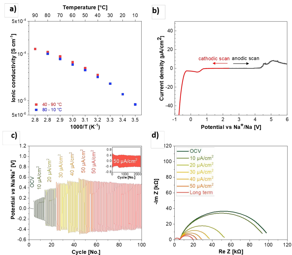
Figure 4. Electrochemical characterization of NaSTFSI-co-PET-MP/4A electrolyte: a) ionic conductivity in the temperature range of 10-90 ^{\circ}\text{C} ; b) anodic and cathodic scan in \text{Na} | \text{Al} cells c) Na stripping/plating test over 2000 h at different current densities in \text{Na} | \text{Na} symmetric cells, and d) the corresponding Nyquist plot after cycling for 10 cycles at each current density. Additionally, the EIS was measured after 100 cycles at 50 \mu\text{A/cm}^2 (red line). All tests were performed at 40 ^{\circ}\text{C} .
