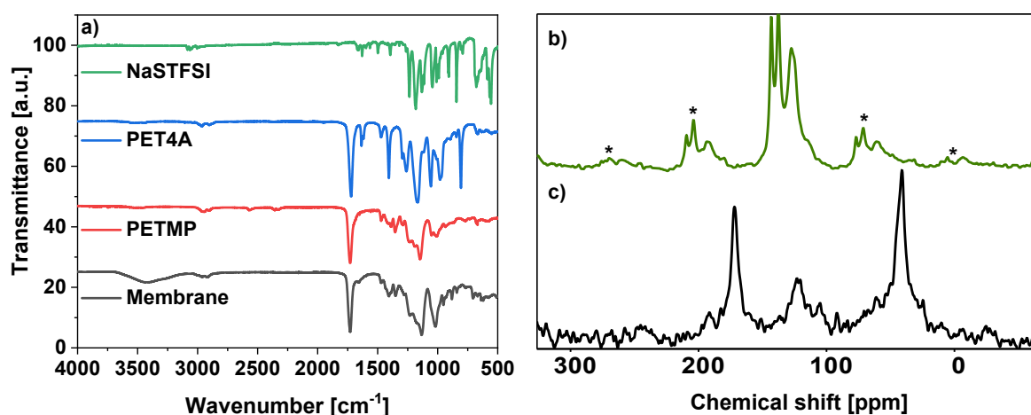
Figure 2. a) FT-IR spectra of NaSTFSI, PET4A, PETMP, and NaSTFSI-co-PET-MP/4A membrane. ^1\text{H} \rightarrow ^{13}\text{C} CPMAS NMR spectrum of b) NaSTFSI and c) NaSTFSI-co-PET-MP/4A electrolyte, recorded at 10 kHz and 14.1 T. Note: Signals marked with asterisks (*) are spinning side-bands.
