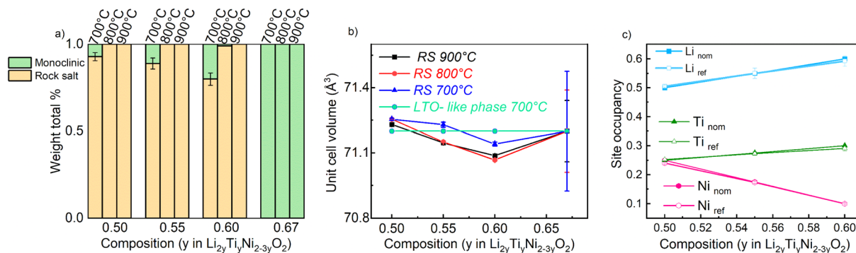
Fig. 4 Evolution of the phase content from Rietveld refinement in the \text{Li}_{2y}\text{Ti}_{1-y}\text{Ni}_{2-3y}\text{O}_2 system. A pure rock salt phase is detected for the samples annealed at 900 °C and 800 °C, while a \text{Li}_2\text{TiO}_3 -like phase appears and grows with increasing y at 700 °C. (b) Unit cell volume of the cubic phases. The value obtained for the \text{Li}_2\text{TiO}_3 -like phase is divided by 6 to account for the larger Z in this structure. (c) Evolution of the site occupancy factors for the samples at 700 °C. Value in (a) and (b) are from refinement of XRD data, while those in (c) from combined refinement of XRD and NPD data.
