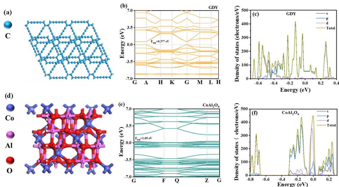
Fig. 13 (a and d) The unit cell of GDY and CoAl 2 O 4 ; (b and e) band structure of GDY and CoAl 2 O 4 ; (c and f) densities of states of GDY and CoAl 2 O 4 .
