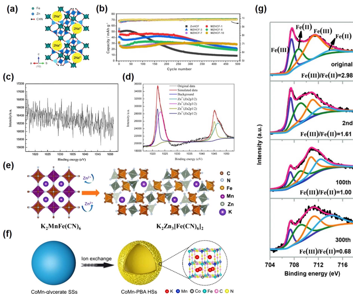
Fig. 10 (a) Unit cell structure of NZH. (Reprinted with permission from ref. 36. Copyright 2012, Royal Society of Chemistry). (b) Cycling performance of ZnHCF and MZHCF at 250 mA g -1 . (Reprinted with permission from ref. 81. Copyright 2021, American Chemical Society). (c) XPS spectra of the original (c) and Zn-inserted CuHCF electrode (d). (Reprinted with permission from ref. 43. Copyright 2014, Elsevier). (e) The schematic diagram of the phase transformation for the KMnHCF electrode. (Reprinted with permission from ref. 50. Copyright 2021, John Wiley and Sons). (f) Synthesis process of CoMn-PBA HSs. (Reprinted with permission from ref. 92. Copyright 2021, John Wiley and Sons). (g) Ex situ XPS spectra of Fe 2p of FeHCF cathodes in the discharge state. (Reprinted with permission from ref. 138. Copyright 2019, John Wiley and Sons).
